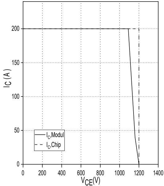
反偏安全工作区 IGBT, 逆变器 (RBSOA) Reverse bias safe operating area IGBT, Inverter (RBSOA) I_C = f(V_{CE}) V_{GE} = \pm 15V, R_{Goff} = 15\Omega, T_{vj} = 150^\circ C
