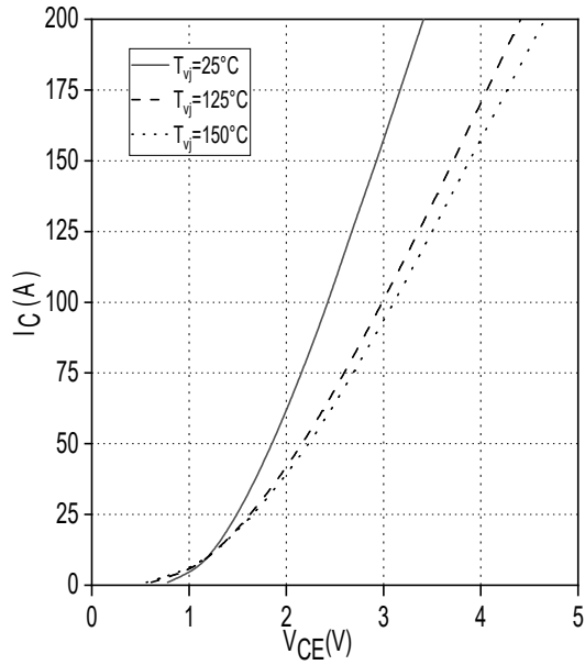
输出特性 IGBT, 逆变器(典型值) Output characteristic IGBT Inverter (typical) I_C = f(V_{CE}) , V_{GE} = 15V
