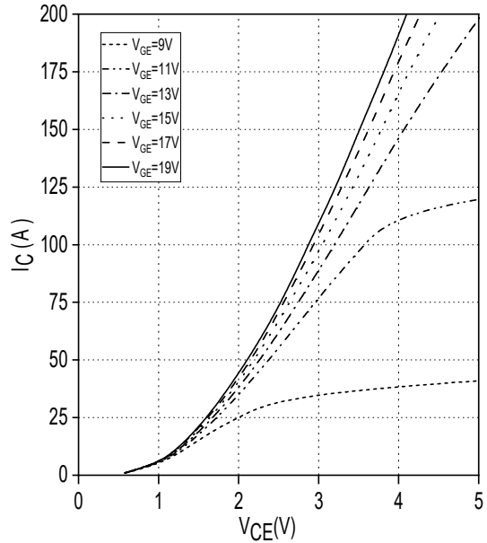
输出特性 IGBT, 逆变器(典型值) output characteristic IGBT Inverter (typical) I_C = f(V_{CE}) , T_{vj} = 150^{\circ}C
