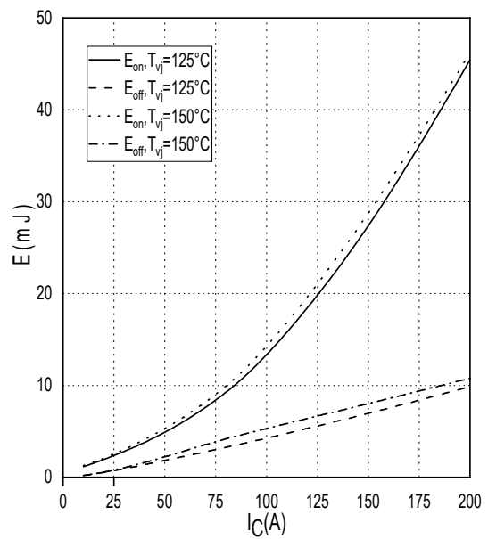
开关损耗 IGBT, 逆变器 (典型值) switching losses IGBT, Inverter (typical) E_{on} = f(I_C), E_{off} = f(I_C), V_{GE} = \pm 15V , R_{Gon} = 4.7\Omega, R_{Goff} = 15\Omega, V_{CE} = 600V
