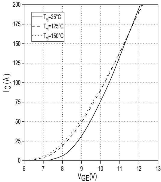
传输特性 IGBT, 逆变器 (典型值) Transfer characteristic IGBT, Inverter (typical) I_C = f(V_{GE}) , V_{CE} = 20V
